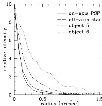
Figure 2. Azimuthally averaged profiles for the on-axis reference star and 3 objects all similar distances from it.
